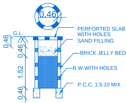
PERCOLATION PIT
