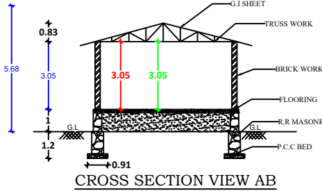
CROSS SECTION VIEW AB
