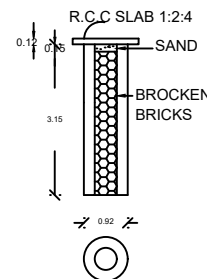
PERCOLATION PIT
