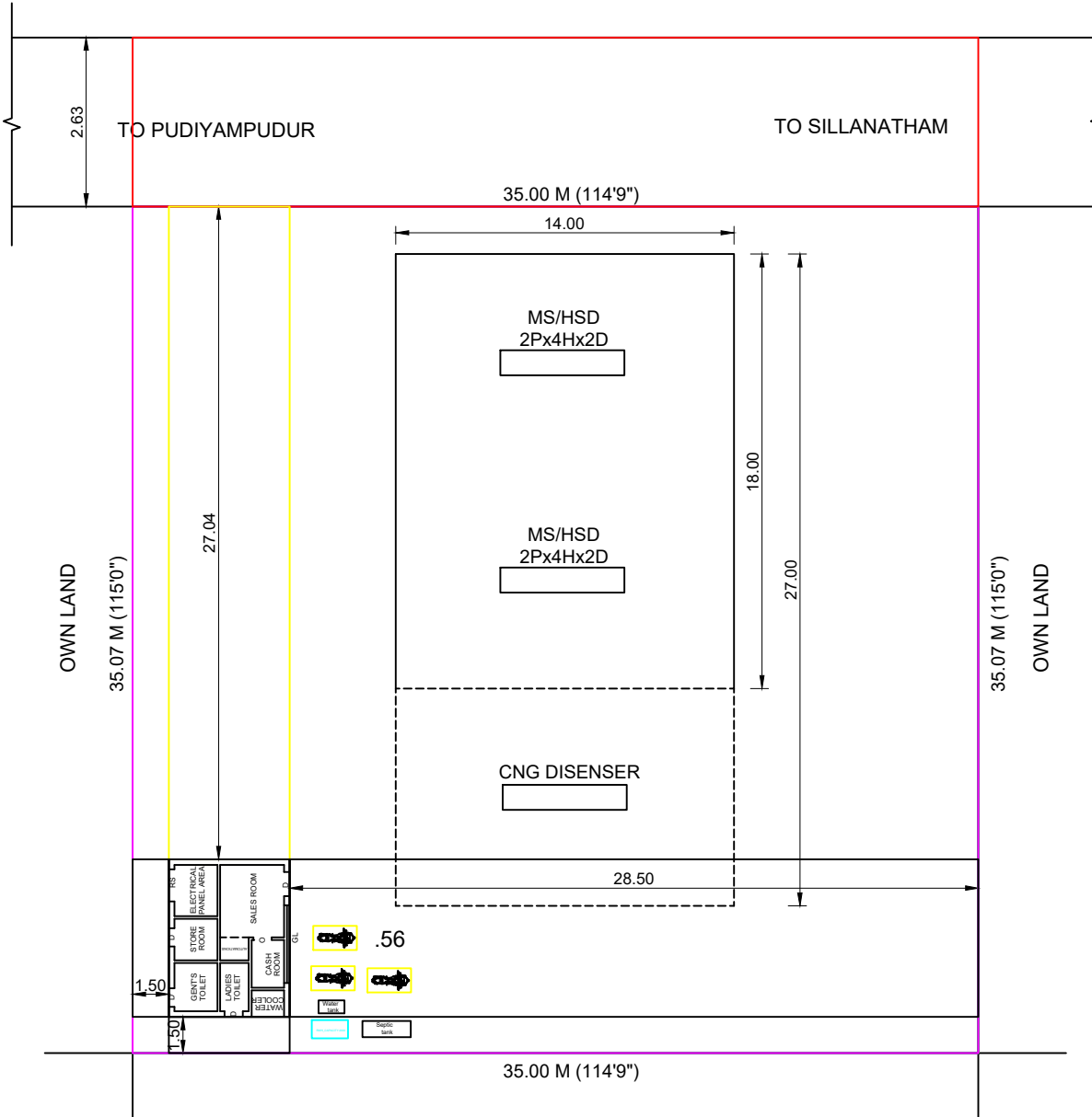
SITE PLAN
