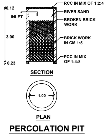
PERCOLATION PIT
