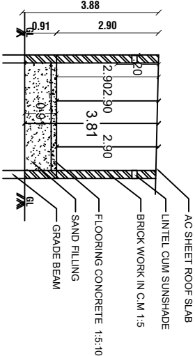
SECTION-AB
