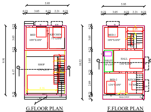
G.FLOOR PLAN
