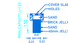
SECTION OF RAIN WATER COLLECTION TANK
