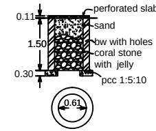
percolation pit
