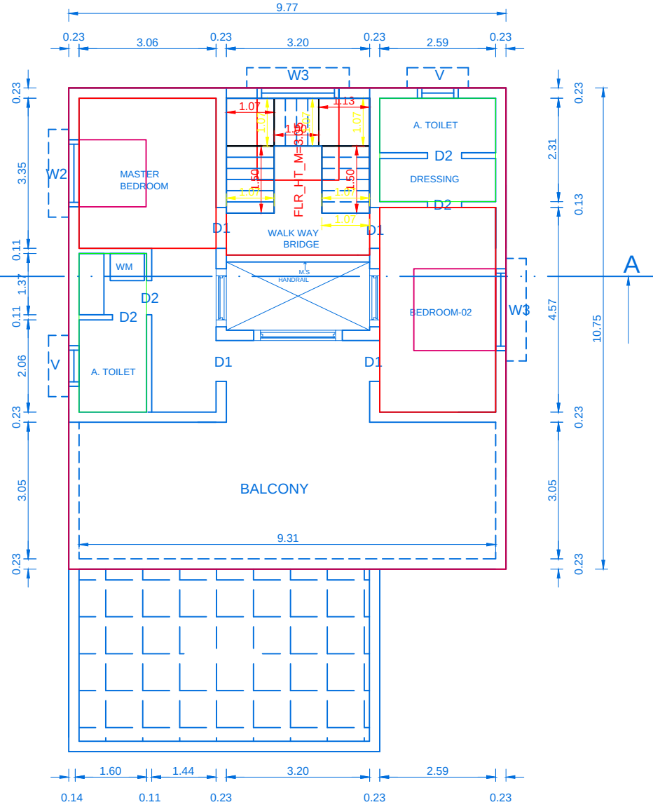
PROP.SECOND FLOOR PLAN
