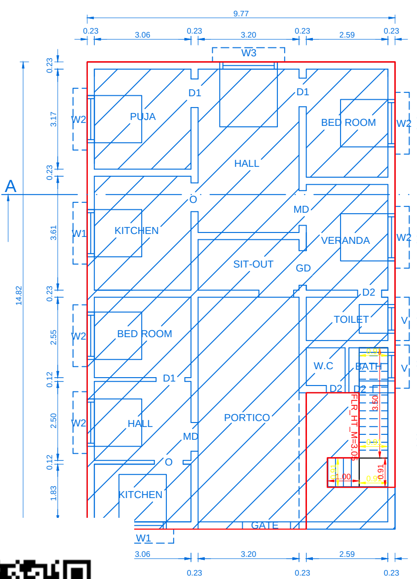
EXG.GROUND FLOOR PLAN
