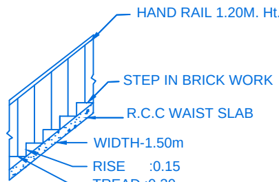
STAIR DETAIL
