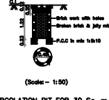
PERCOLATION PIT FOR 30 Sq. m.
