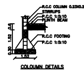
COLUMN DETAILS
