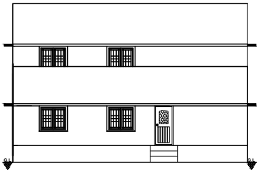
ELEVATON
