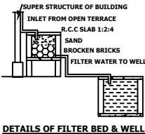
DETAILS OF FILTER BED & WELL
