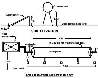
SOLAR WATER HEATER PLANT
