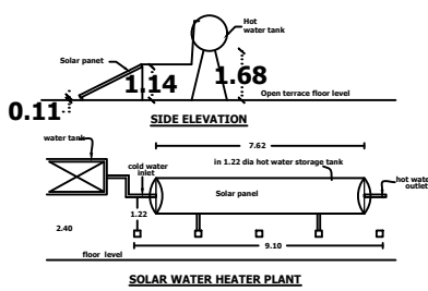
SOLAR WATER HEATER PLANT
