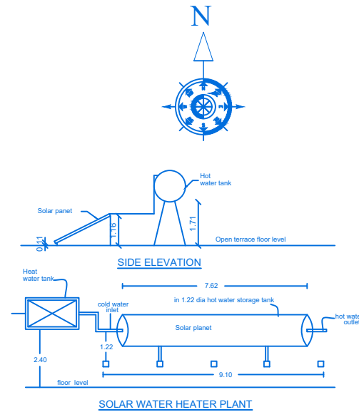
SOLAR WATER HEATER PLANT
