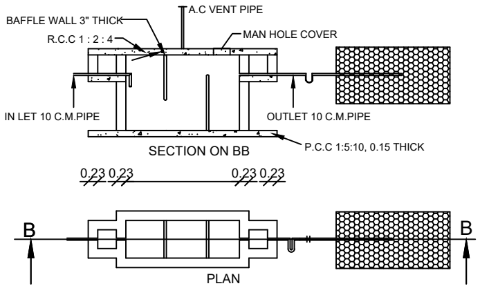
SEPTIC TANK AND TRENCH & U TRAP ADOPTED
