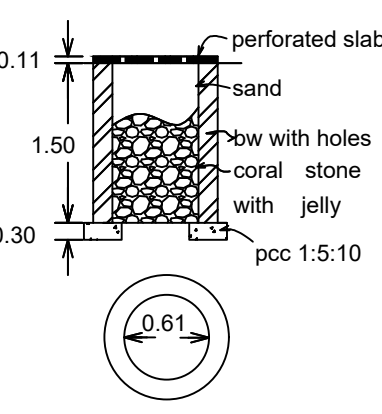
PERCOLATION PIT
