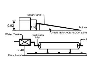
Details of solar water heating system
