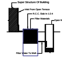
Details Of Rainwater Harvesting System
