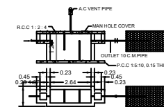
SEPTIC TANK DETAILS
