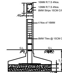
RCC COLUMN DETAILS
