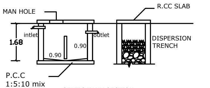
SEPTIC TANK SECTION
