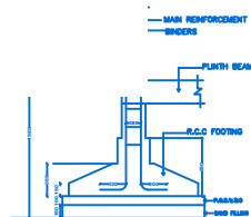
TYPICAL SECTION OF R.C.C COLUMN FOUNDATION SCALE 1"=2'-0"
