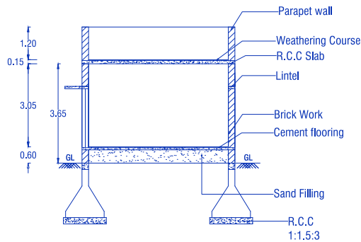
CROSS SECTION ON 'AB'
