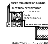
RAINWATER HARVESTING
