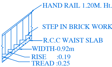
STAIR DETAIL
