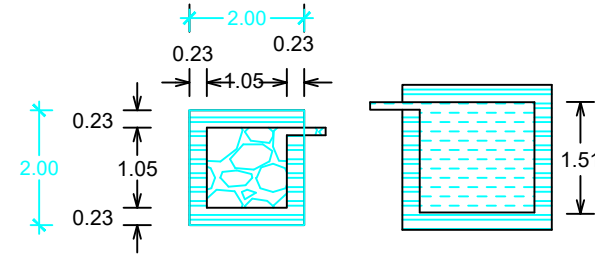
RWH_CAPACITY_L=1000LTRS DETAILS OF FILTER BED & WELL
