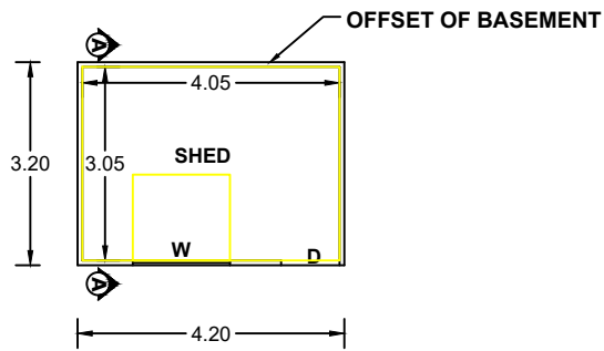
PLAN EAST FACING SHED
