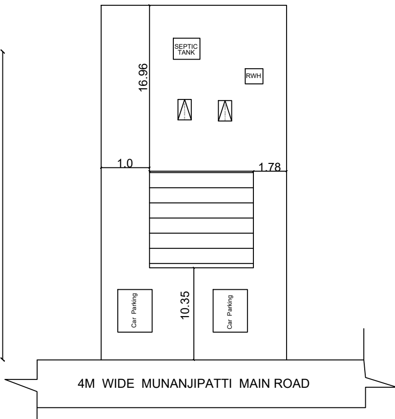
SITE PLAN
