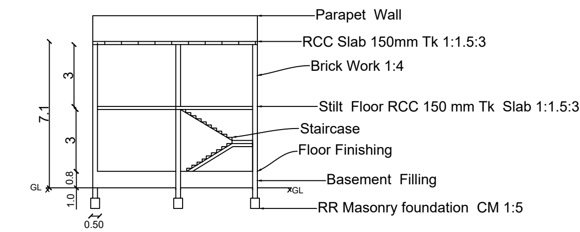
SECTION A-A VIEW
