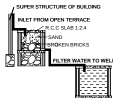
RAINWATER HARVESTING
