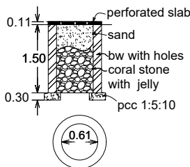
percolation pit
