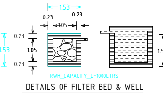
DETAILS OF FILTER BED & WELL
