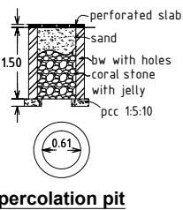
percolation pit
