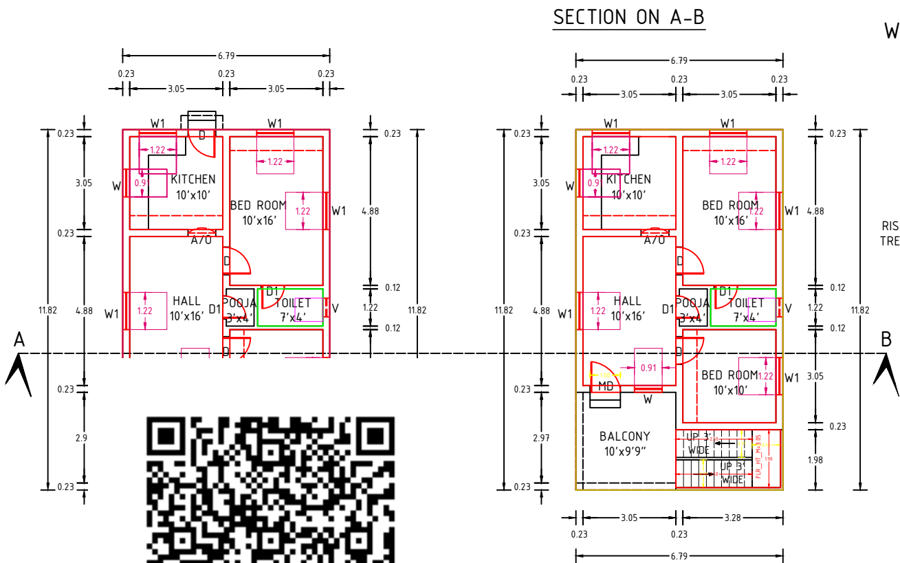
PROP. FIRST FLOOR PLAN
