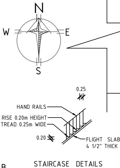
STAIRCASE DETAILS
