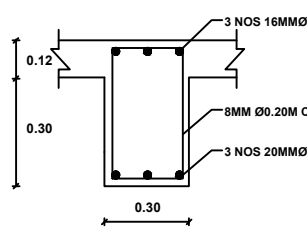
ROOF BEAM DETAILS
