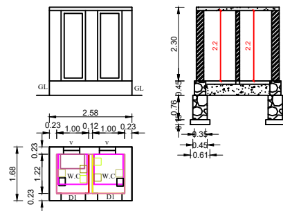
BATHROOM PLAN
