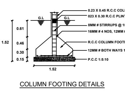
COLUMN FOOTING DETAILS
