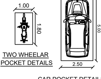
CAR POCKET DETAILS
