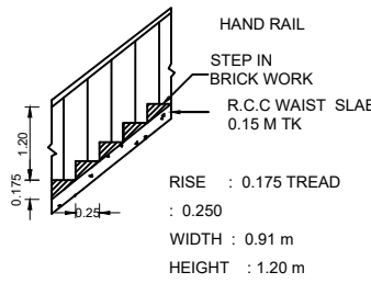
STAIR DETAILS
