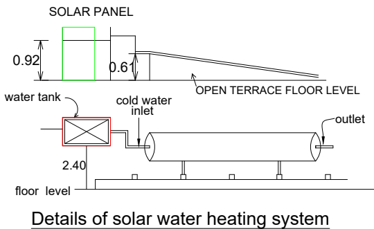
Details of solar water heating system
