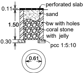
percolation pit
