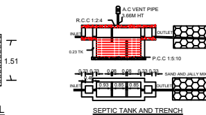
SEPTIC TANK AND TRENCH
