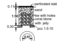
percolation pit
