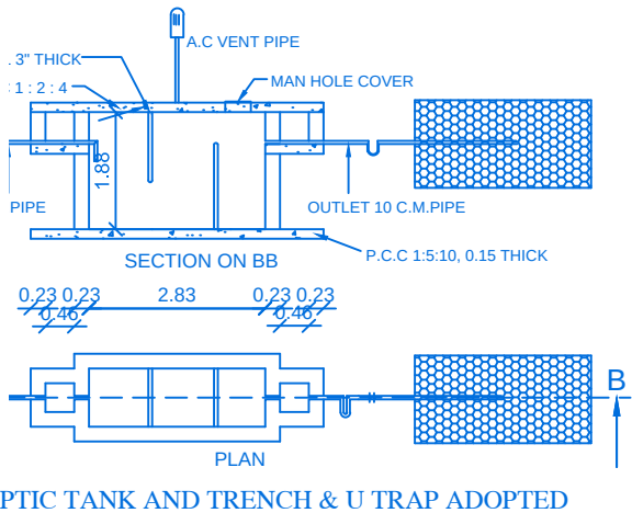
SEPTIC TANK AND TRENCH & U TRAP ADOPTED
