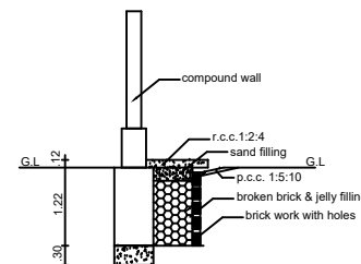
PLINTH BOUNDARY PERCOLATION PIT
