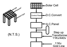
SOLAR SYSTEM FLOW DIAGRAM
