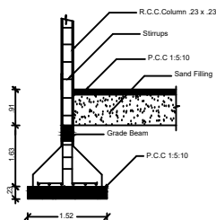
COLUMN DETAIL
