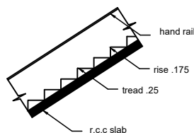
STAIR
