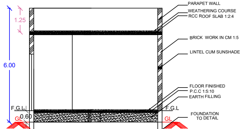
SECTION "A-B"
