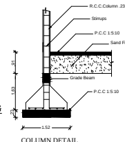
COLUMN DETAIL
