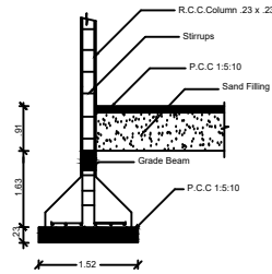
COLUMN DETAIL
