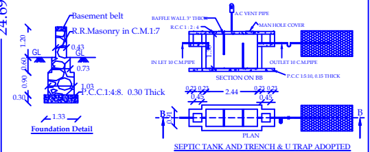
SEPTIC TANK AND TRENCH & U TRAP ADOPTED
