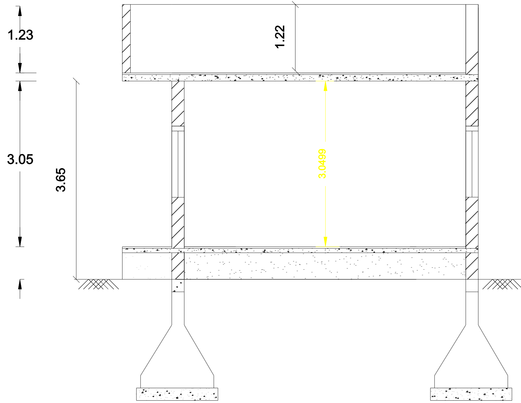
CROSS SECTION ON 'AB'
