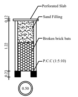
DRAINAGE SOAK PIT DETAILS
