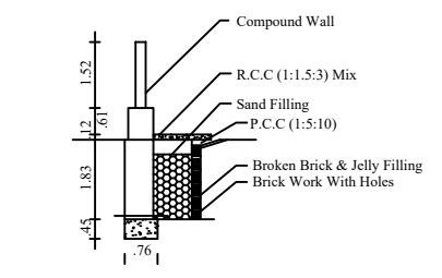
RAIN WATER HARVEST DETAILS
