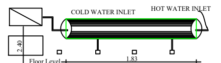
DETAILS OF SOLAR HOT WATER SYSTEM
