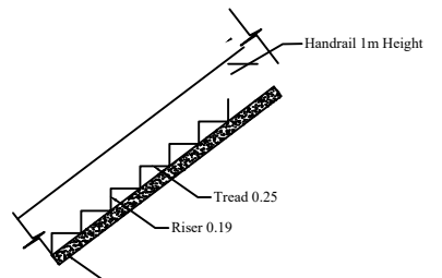
STAIR DETAILS
