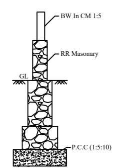
DETAILS OF RR MASONARY
