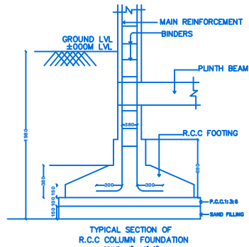
SCALE : 1" = 2'-0"
