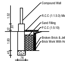
RAIN WATER HARVEST DETAILS
