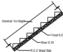
STAIR DETAILS
