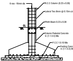
COLUMN FOOTING DETAILS
