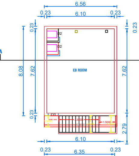
GROUND FLOOR PLAN(BLOCK-2)
