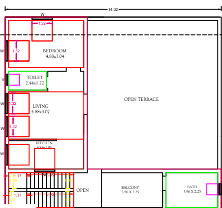
RO.FIRST FLOOR PLAN
