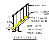
STAIR DETAILS
