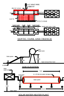
SOLAR WATER HEATER PLANT
