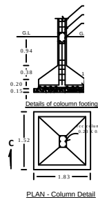
PLAN - Column Detail
