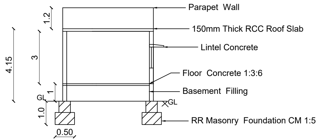
SECTION A - A VIEW
