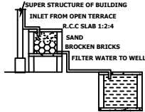
DETAILS OF FILTER BED & WELL
