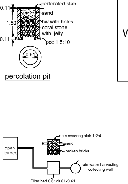
DETAILS OF RAIN WATER HARVESTING SYSTEM
