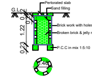
PERCOLATION PIT FOR 30 Sq. m. (Scale:- 1:50)
