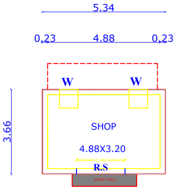
SHOP PLAN
