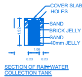
SECTION OF RAIN-WATER COLLECTION TANK
