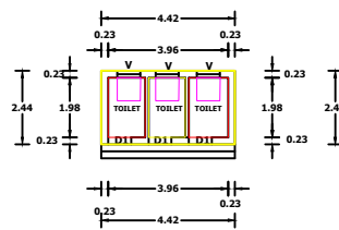
PRO. TOILET PLAN
