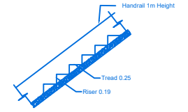
STAIR DETAILS
