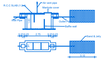
SEPTIC TANK & TRENCH
