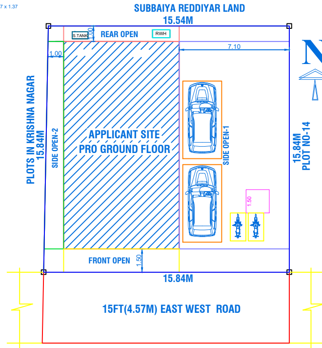
SITE PLAN(1:100)
