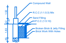
ATER HARVEST DETAILS
